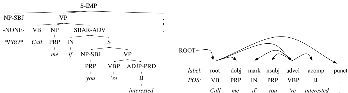
Figure 1: Example constituency and dependency trees. As is common practice in constituency parsing, function labels and empty nodes were available at training time but were not included in the evaluation.
