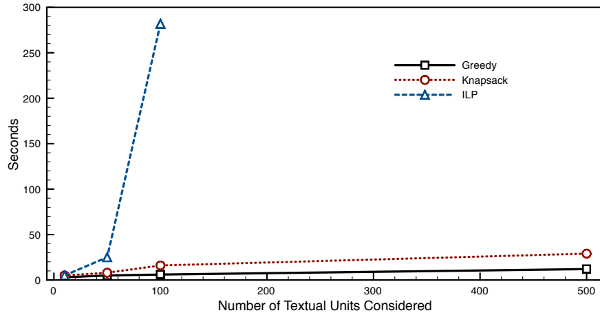
Fig. 3. Plots average number of seconds to summarize a document collection as a function of the number of textual units considered.
